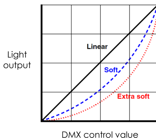
Figure 3. Dimming curves
