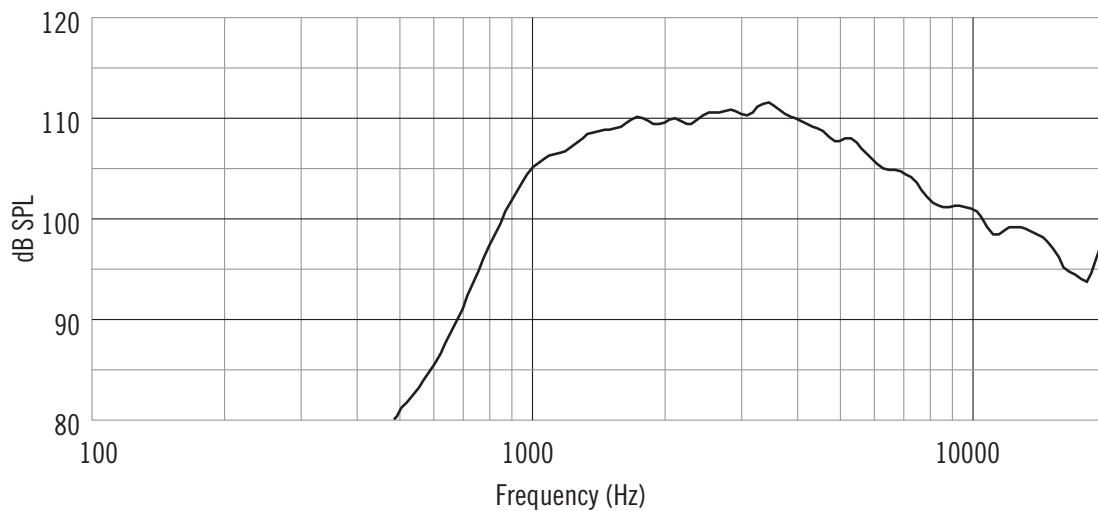
Response 1W/1m
