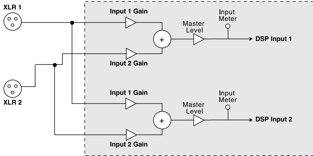
INPUT DIAGRAM
