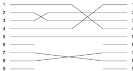
DB-9 female-to-female null modem cable
