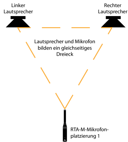
Level Assist/AutoEQ-Mikrofonposition 1
